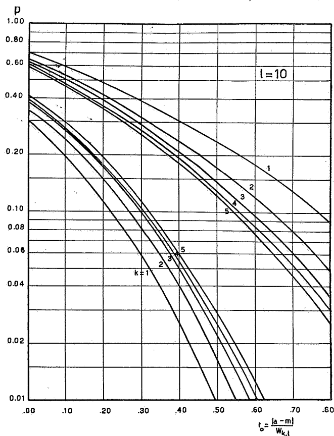
Fig. 1. Central confidence intervals for the percentage defectives in a normal distribution with confidence-coefficient
